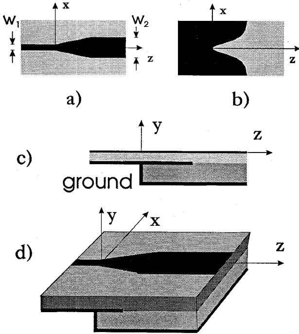
Fig. 3. Different perspectives of the smooth transition. (a) Top view of the upper metallized interface (strip interface). (b) Top view of the lower interface (slot interface). (c) Longitudinal side view of the smooth interface. (d) Three-dimensional view.
