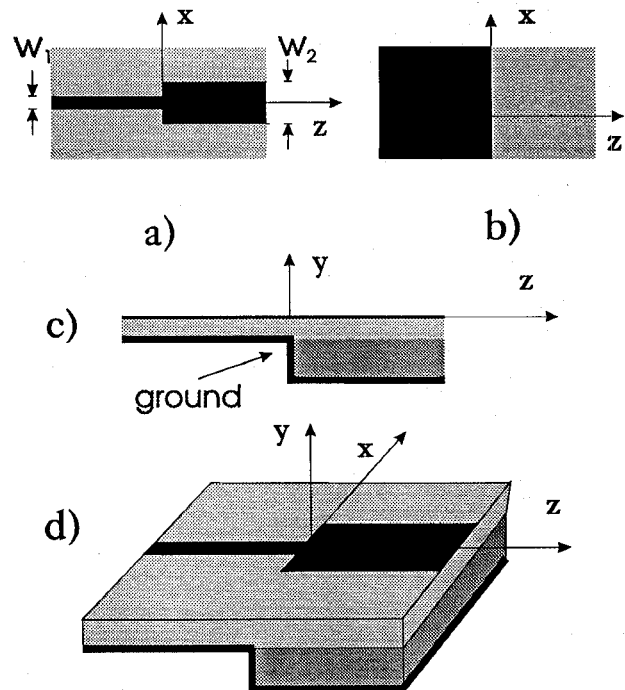
Fig. 1. Different perspectives of an abrupt transition between single- and double-layer microstrips. (a) Top view of the strip pattern on the upper side of the upper substrate. (b) Ground metallization of the bottom side of the upper substrate. (c) Side view of the abrupt transition. (d) Three-dimensional view.
