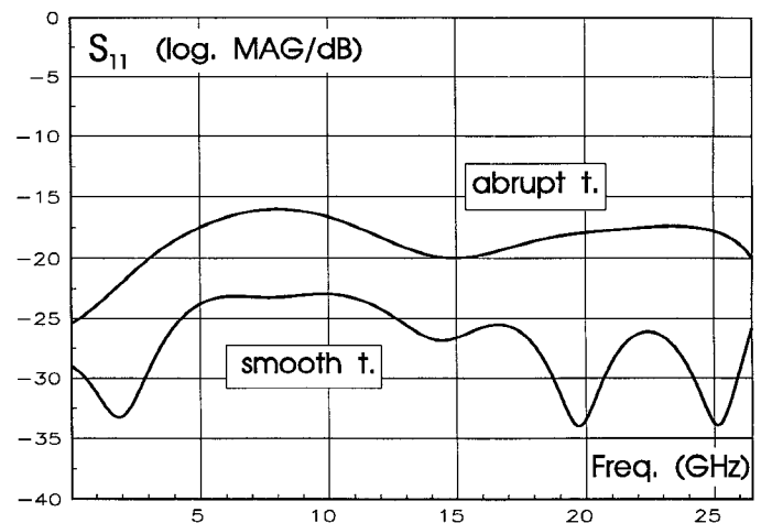
Fig. 7. Comparison of the S_{11} -response for the abrupt and smooth transitions.
